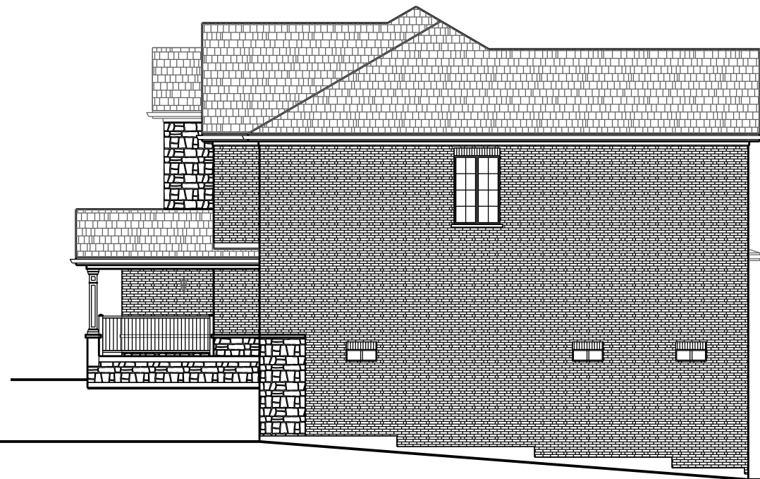
Right Side ( North ) Elevation
